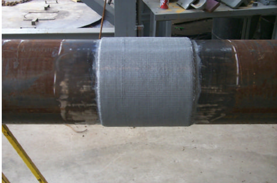
Figure 6 Completed installation of Armor Plate Pipe Wrap
