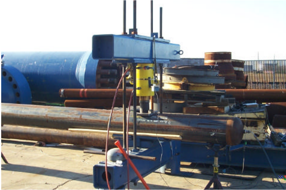
Figure 1 Dent installation rig used to install dents
